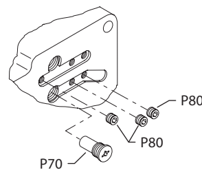
VIEW "A" END CAP GASKET FACE
