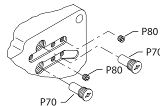
VIEW "A" END CAP GASKET FACE RIGHT HAND ROTATION
