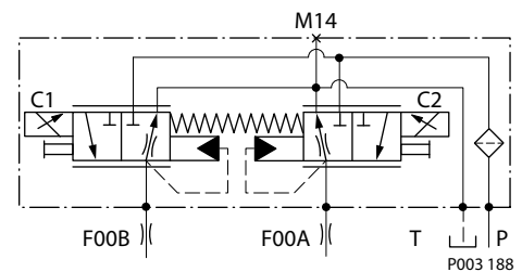
NFPE schematic
