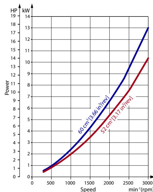
Charge pump power requirements
