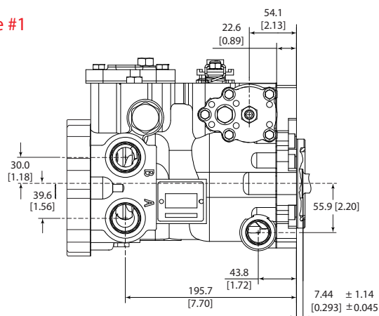
Bottom view (with MDC and suction filtration)
